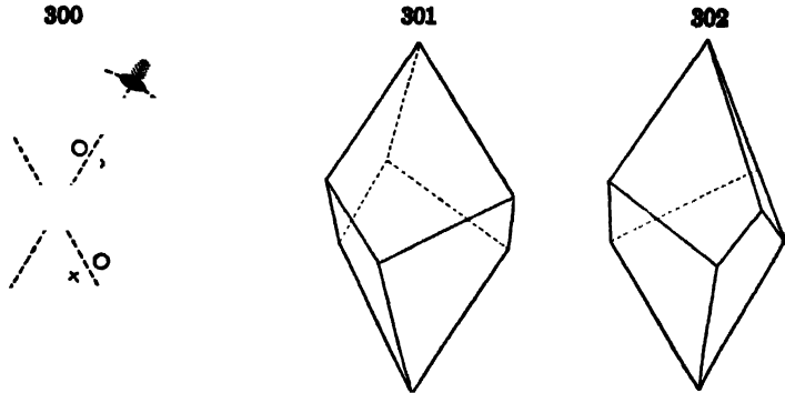
Symmetry of Trapezohedral Class
